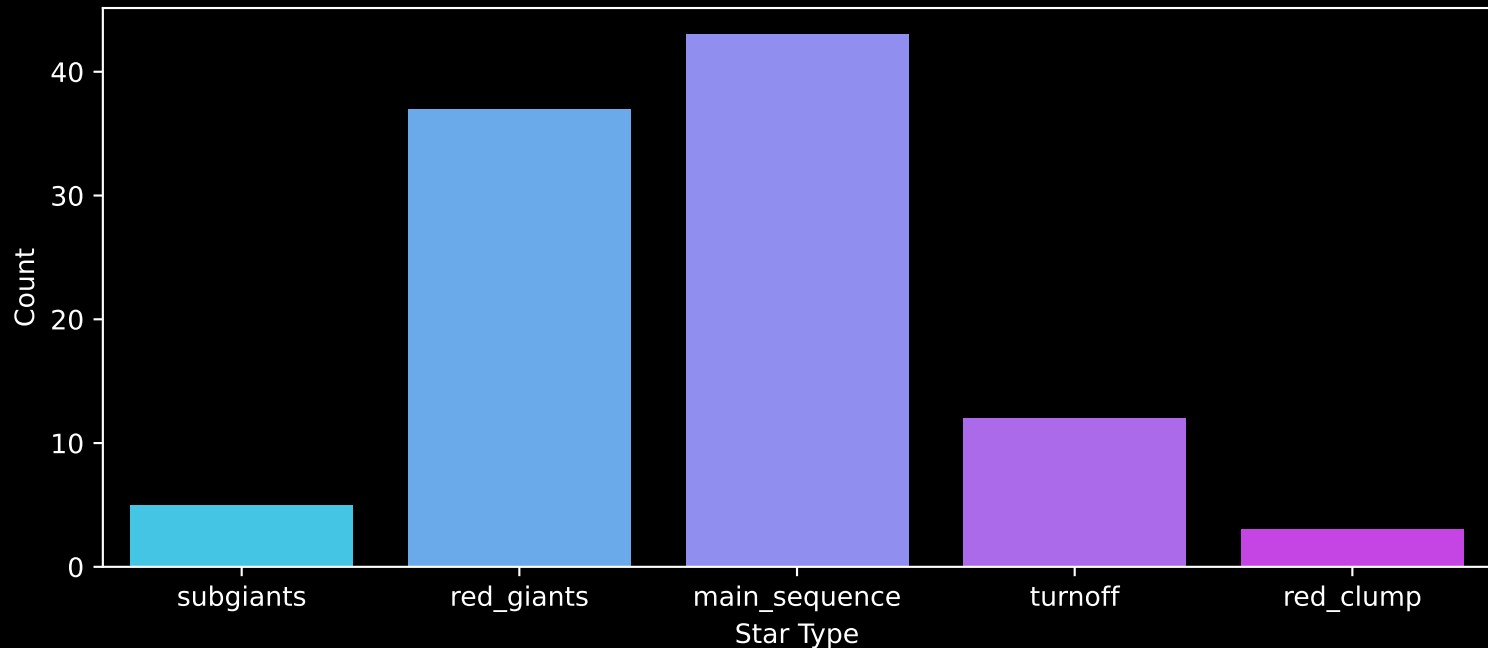
APOGEE DR17 Field: [GALCEN] Count plot of Star Type
