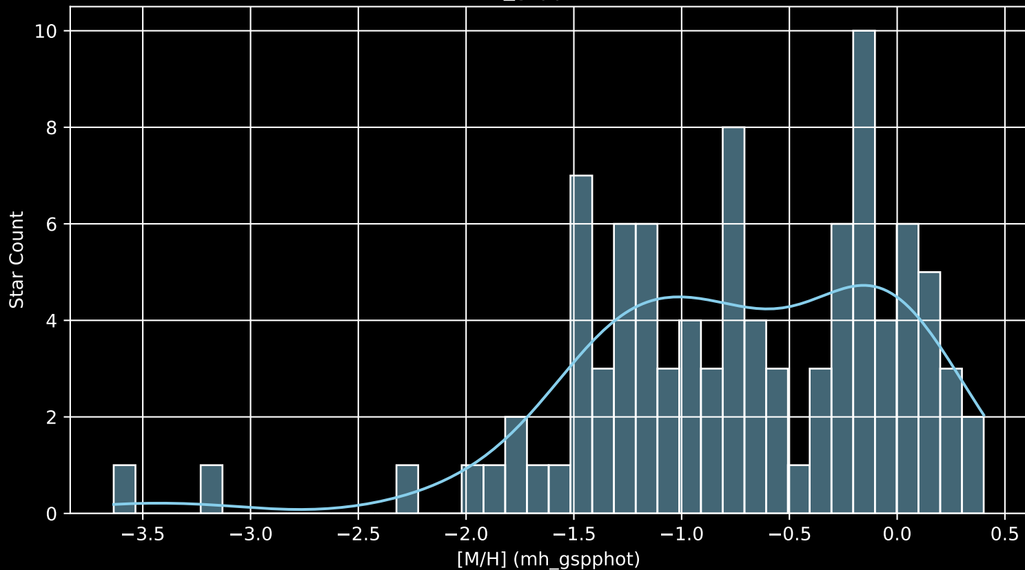
APOGEE DR17 Field: [GALCEN [M/H] (mh_gspphot) (n= 96)
