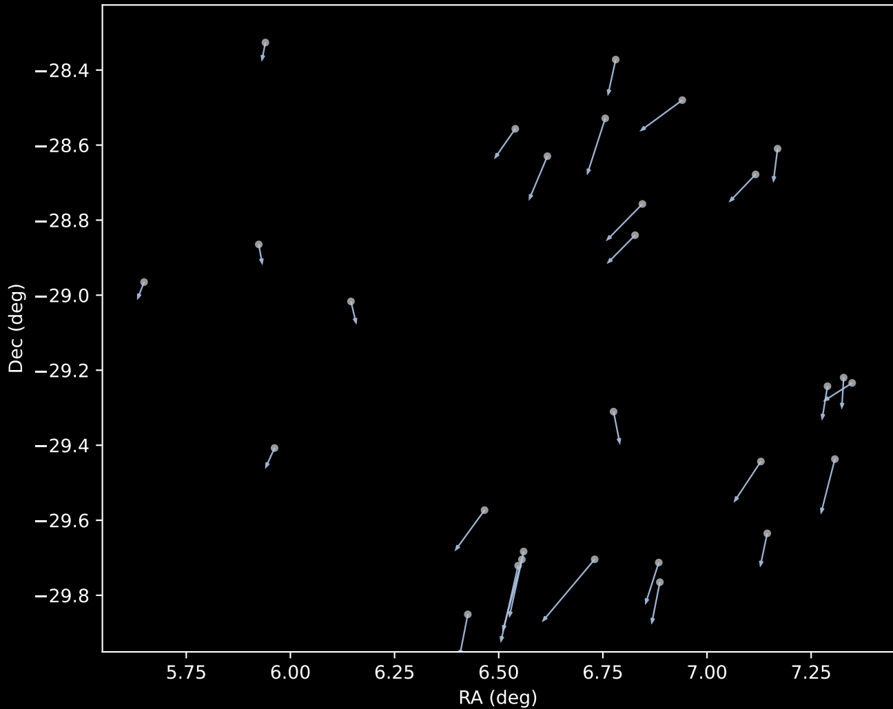
APOGEE DR17 Cluster 1 Proper Motion Vectors (n=29)
