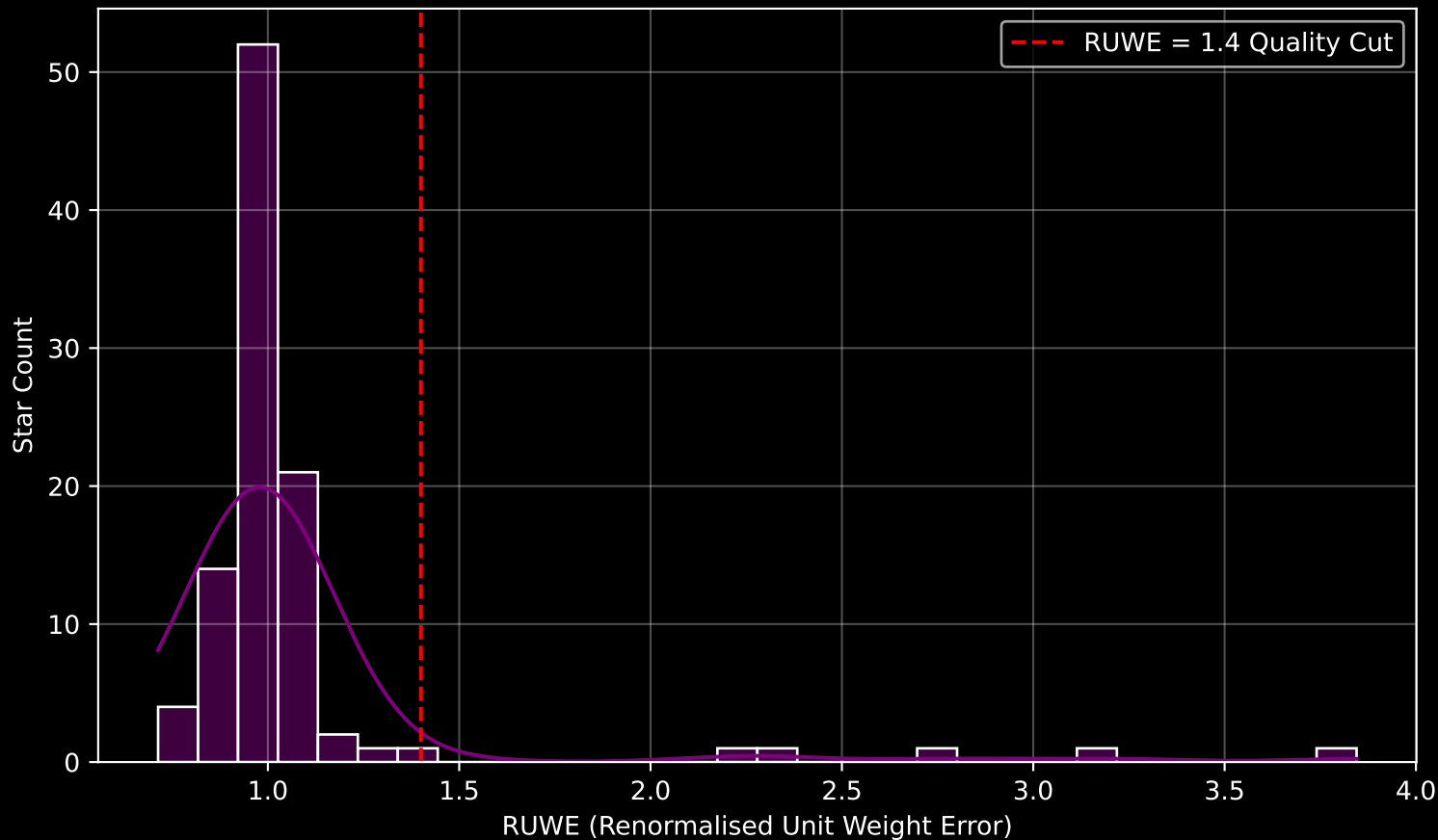
GAPOGEE DR17 Field [GALCEN] RUWE Distribution (n= 100)
