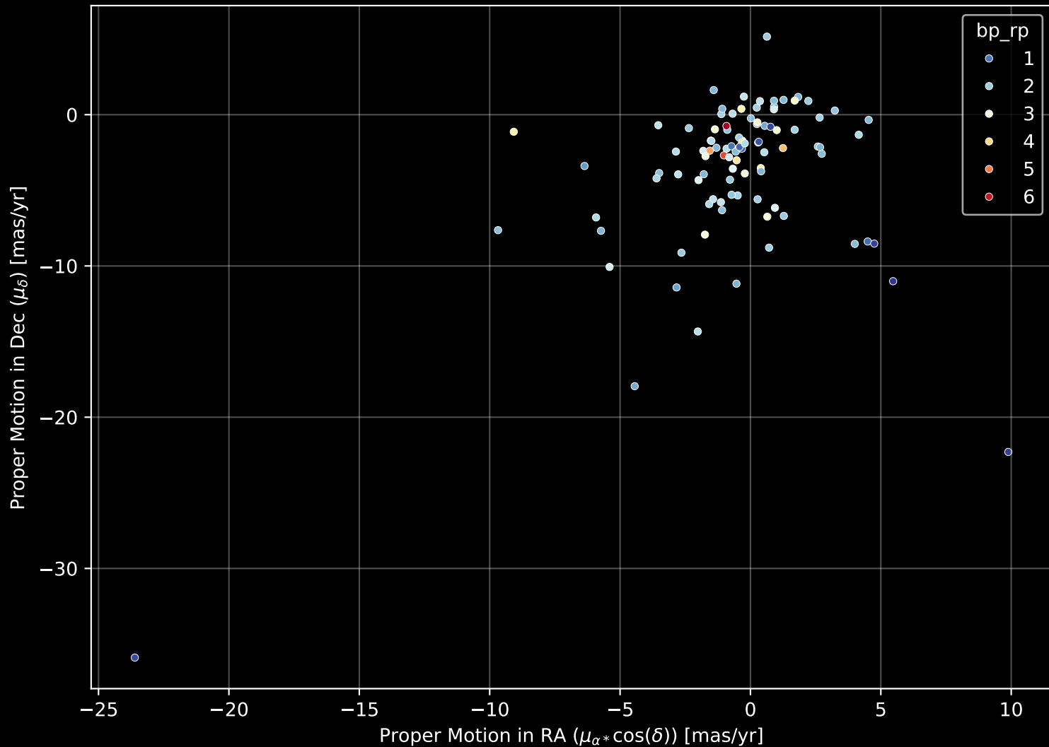
APOGEE DR17 Field: [GALCEN] Proper Motion Diagram (n= 100)
