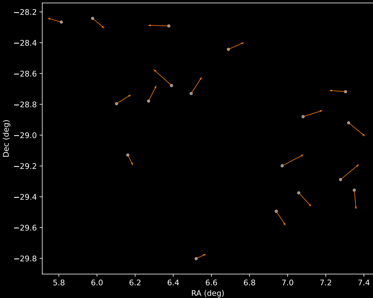
APOGEE DR17 Cluster 2 Proper Motion Vectors (n=18)
