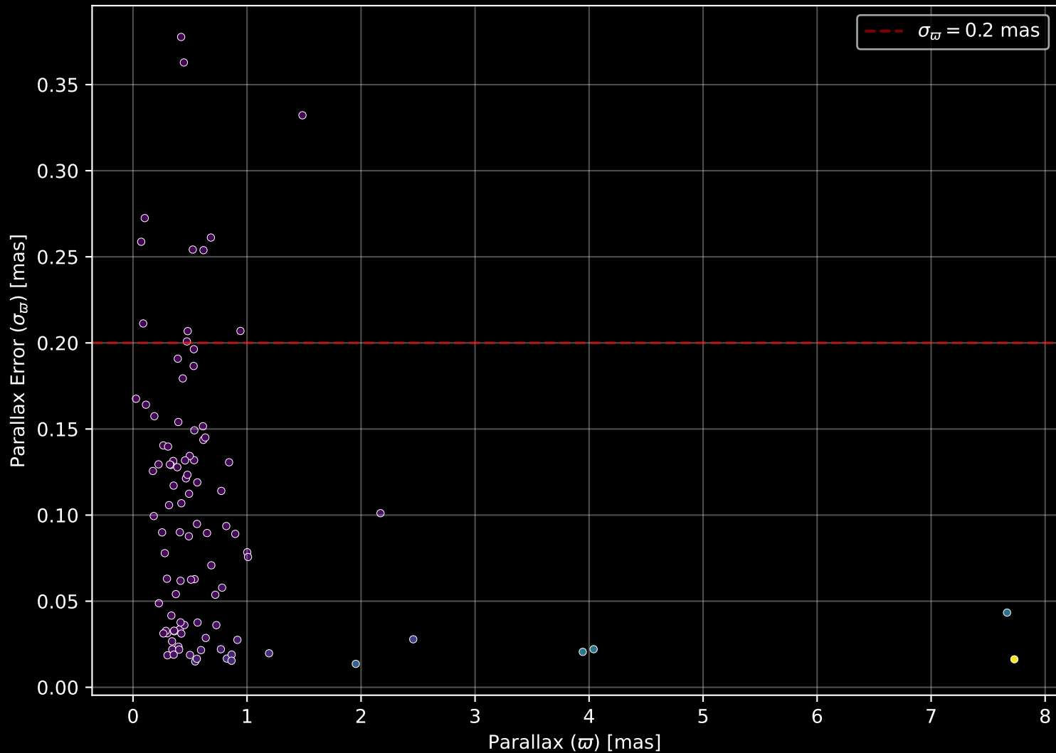
APOGEE DR17 Field: [GALCEN] Parallax Quality (n= 100)
